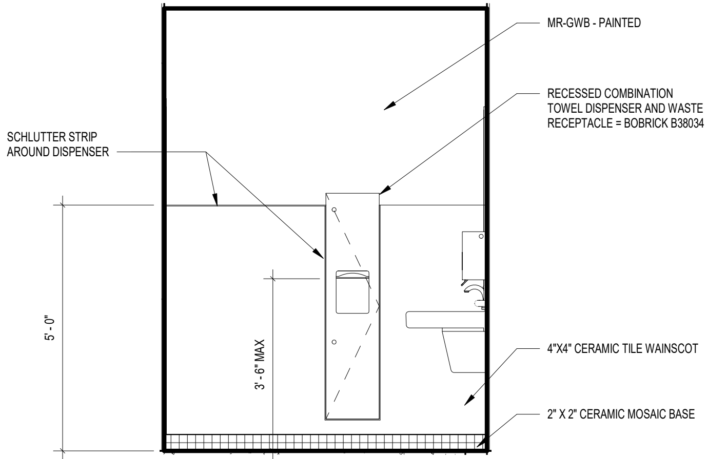
① TOILET - EAST - AMENDED PERMIT 1/2" = 1'-0"
